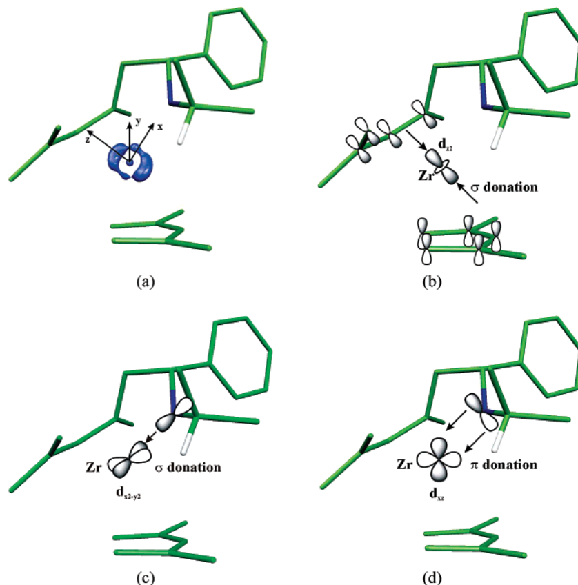
Figure 6. Three-dimensional representation of (a) the static deformation density around Zr atom for model III and schematic representation of the (b) Zr ← diene \sigma donation, (c) Zr ← N \sigma donation, and (d) Zr ← N \pi donation. Isocontour of 0.2 e \text{ \AA}^{-3} (positive in blue).
