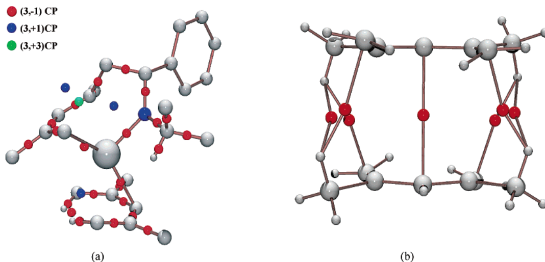
Figure 4. Localization of the critical points of the electron density in (a) the Zr coordination sphere and (b) the interdimer region. Only relevant critical points are depicted.
