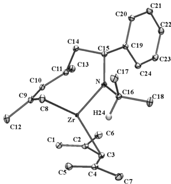
Figure 1. ORTEP view and atom numbering scheme of Zr(2,4-C 7 H 11 )(NM 2 -CHPhCH 2 CMe=CHCMe=CH 2 ). Ellipsoids drawn at the 50% level probability and arbitrary radius for H24. H atoms (except H24) omitted for clarity.
